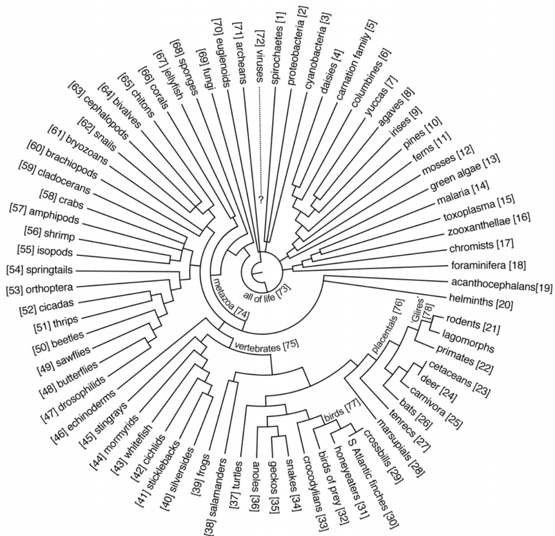
Supplementary Figure 1. The 78 “adaptive radiations” reflected in this tree come from the recent phylogenetic literature, and show that “adaptive radiation” is a metaphor that has given a powerful heuristic to biologists working on all groups of organisms at all levels of the phylogenetic hierarchy. More importantly, it unites the nearly 300 authors of these studies with a common theme.
